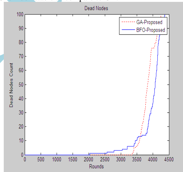
Figure 6.9. Graph showing comparison of dead nodes after each round using GA-Proposed and BFO-Proposed
