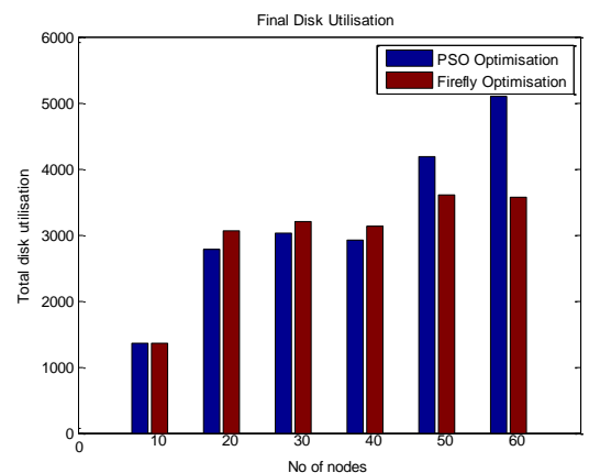
Figure 4: final disk utilisation comparative bar plot
